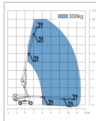
作业曲线图 Work Curve Graph
